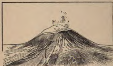
FIG. 134.—The central cone of Vesuvius as it appeared after the eruption of 1906, but with the earlier profile indicated. The truncation represents a lowering of the summit by some five hundred feet, with corresponding increase in the diameter of the crater (after Johnston-Lavis).
